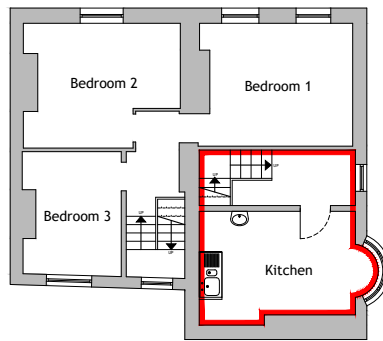
+02 Second Floor Plan
