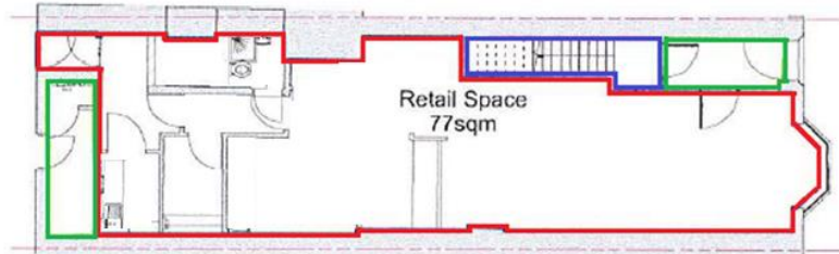
Proposed Ground Floor Scale - 1:200
